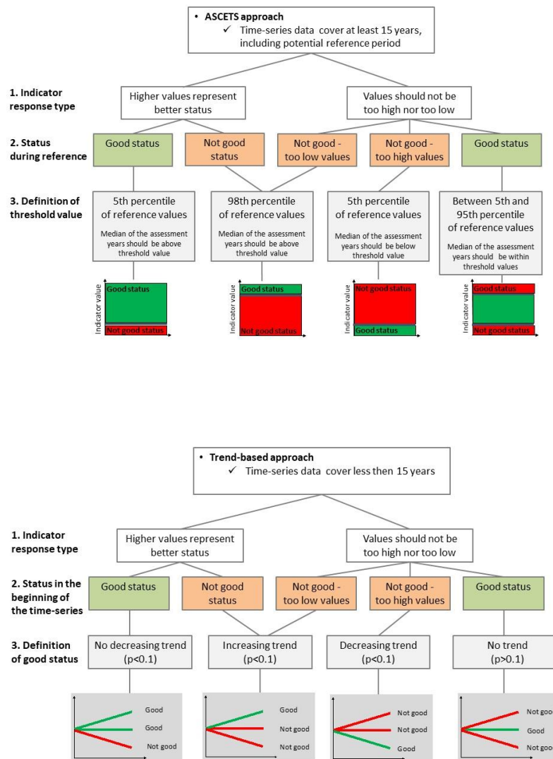
Figure 6. Decision tree for assessment using coastal fish community structure. The ASCETS approach (top figure) and trendbased approach (bottom figure) are presented.
