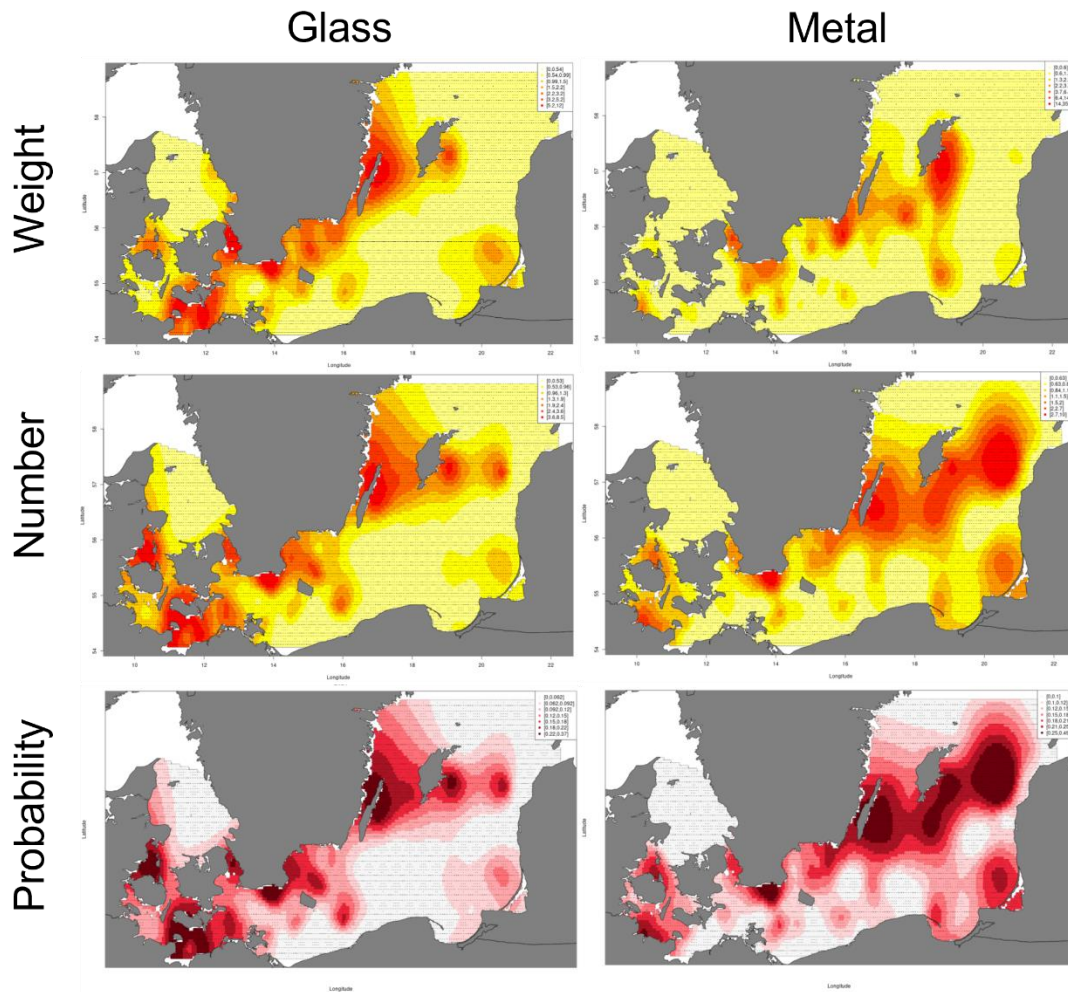
Figure 4a. Distribution of different litter types in weight, number and probability of catching litter. Colouring reflects amount relative to the mean, yellow/white is low amounts, red/dark red is high amounts. Note the limited sampling in deeper areas, see figure 3, and that the areas presented are not directly compatible with the standard HELCOM Assessment Units.
