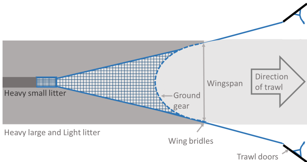
Figure 5. The active region of a benthic trawl net for light and heavy litter. Text indicates the types of litter not retained in each part of the trawl path. All litter except very small items are retained in the darkest grey part of the trawl path.
