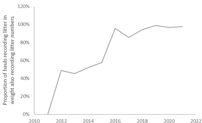
Figure 7. Development in the proportion of hauls recording litter in weight where number of litter items is also recorded.
