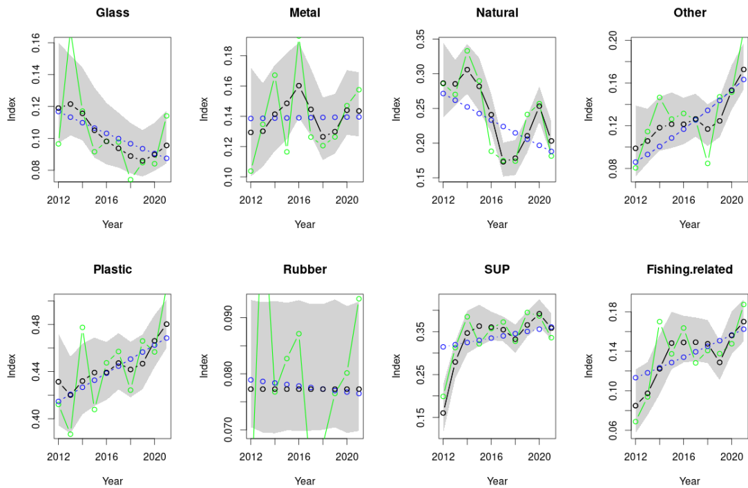
Figure 3. Temporal development in probability of catching litter as estimated by models 1 (black, grey is 95% confidence interval of the estimate), 2 (green) and 3 (blue). Top row from left to right: glass, metal, natural, other. Bottom row from left to right: plastic, rubber, SUP, fisheries related plastic. Note difference in scale of the y-axis.
