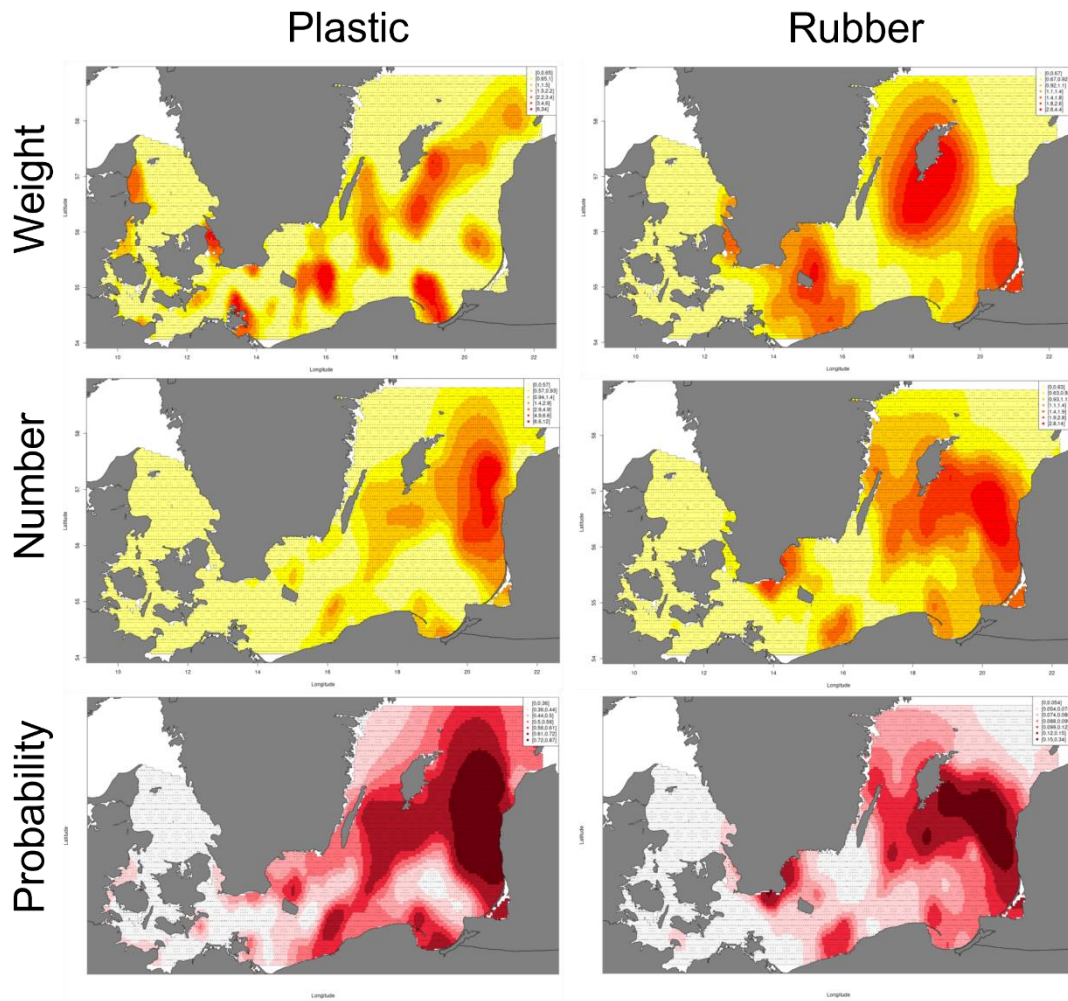
Figure 4c. Distribution of different litter types in weight, number and probability of catching litter. Colouring reflects amount relative to the mean, yellow/white is low amounts, red/dark red is high amounts. Note the limited sampling in deeper areas, see figure 3, and that the areas presented are not directly compatible with the standard HELCOM Assessment Units.
