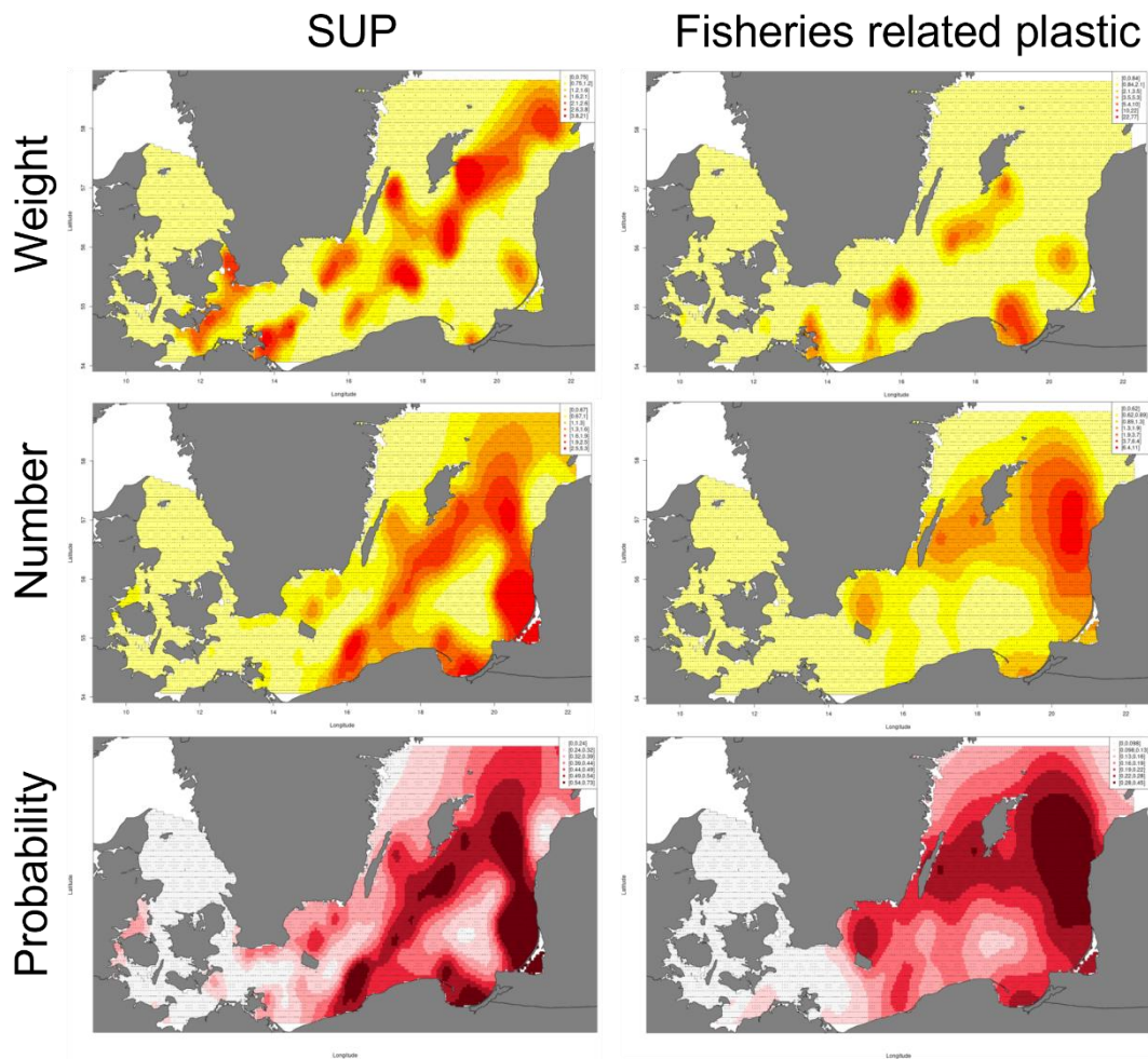
Figure 4d. Distribution of different litter types in weight, number and probability of catching litter. Colouring reflects amount relative to the mean, yellow/white is low amounts, red/dark red is high amounts. Note the limited sampling in deeper areas, see figure 3, and that the areas presented are not directly compatible with the standard HELCOM Assessment Units.
