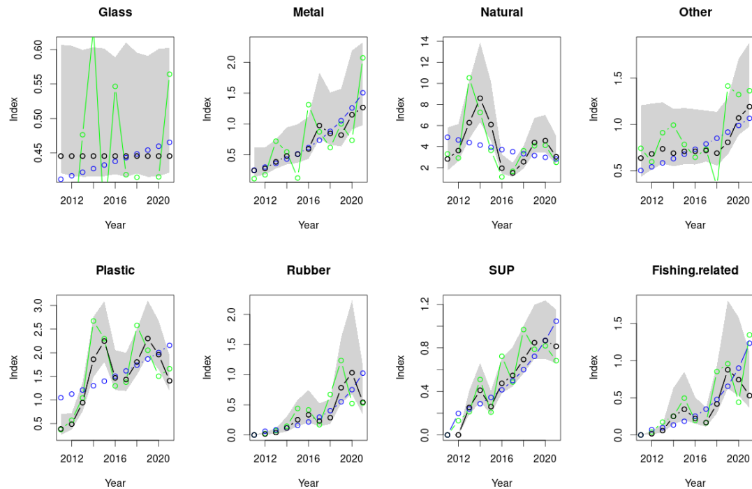
Figure 1. Temporal development in kg litter/km 2 as estimated by models 1 (black, grey is 95% confidence interval of the estimate), 2 (green) and 3 (blue). Top row from left to right: glass, metal, natural, other. Bottom row from left to right: plastic, rubber, SUP, fisheries related plastic. Note difference in scale of the y-axis.
